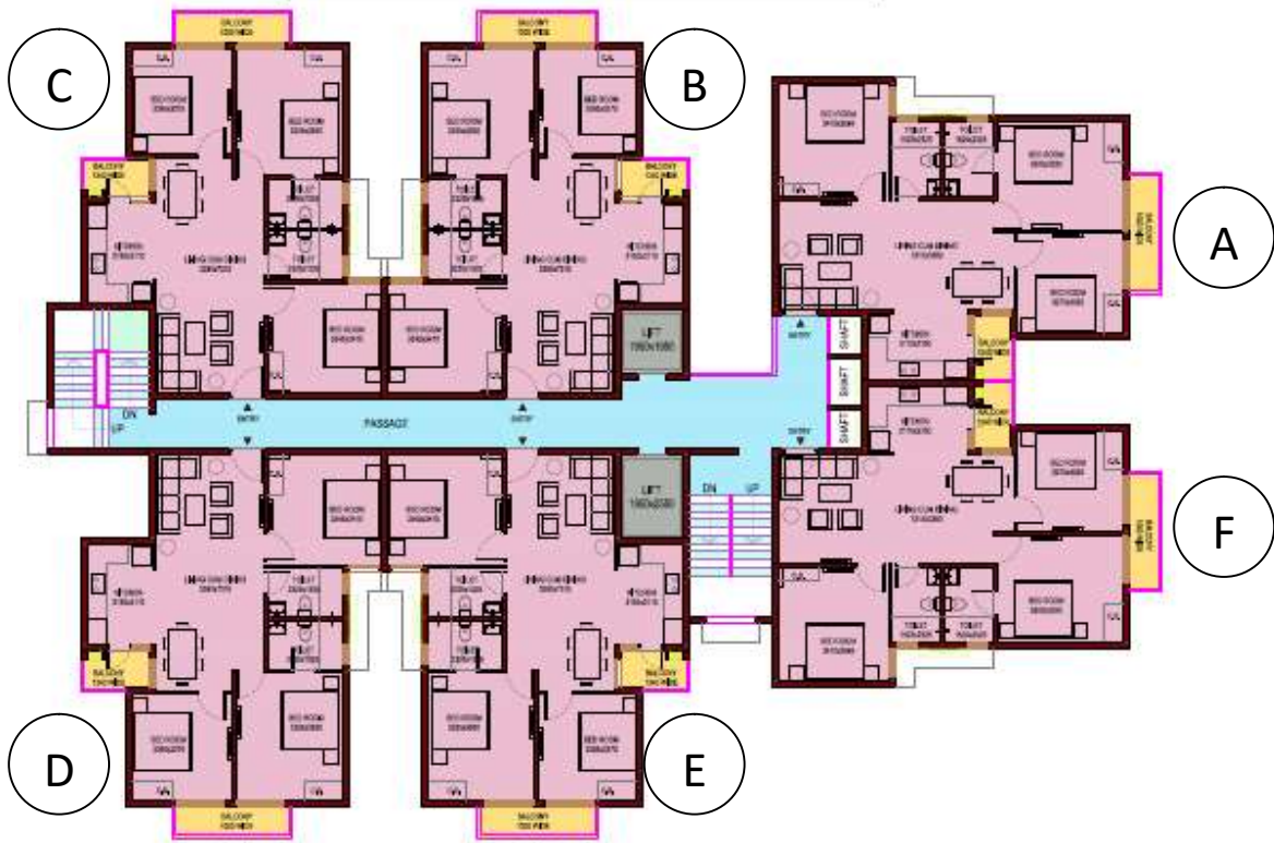
TITLE - FLOOR PLAN OF HIG TOWER UD LAND SITE (PROPOSED)
