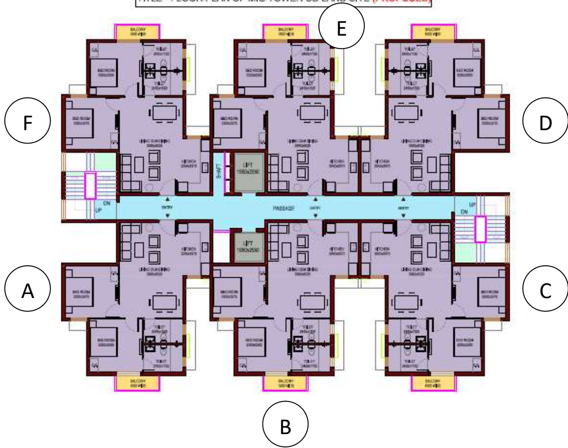
TITLE - FLOOR PLAN OF MIG TOWER UD LAND SITE (PROPOSED)
